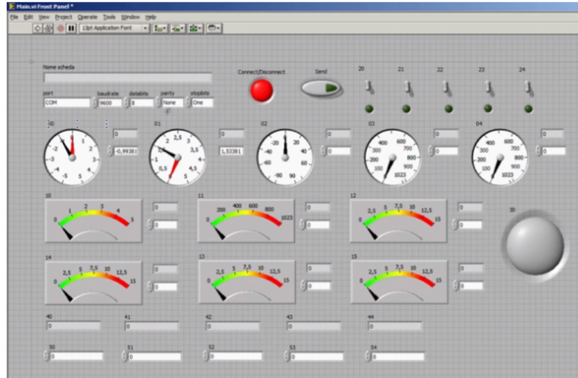
Figure 10. LabView GUI [19]
