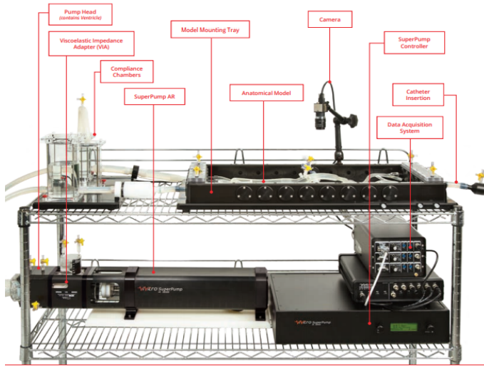
Figure 1. Vivitro Labs Complete System [27]
