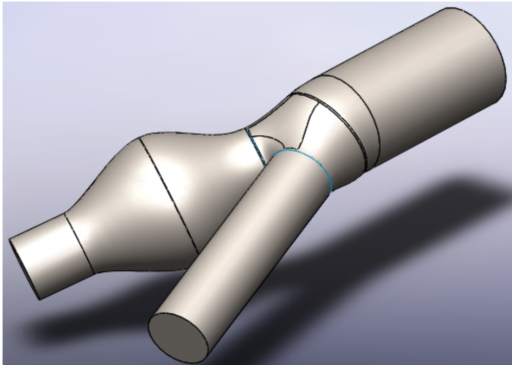
Figure 20: Solidworks Model of Exterior Mold in Accordance with a 4mm Wall Thickness
