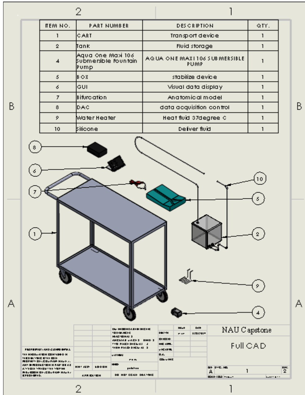
Figure 26: Exploded CAD model with atlas
