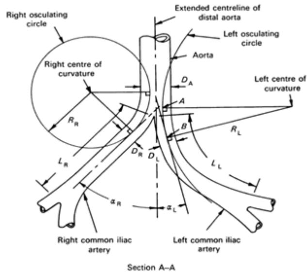
Figure 17: Geometry of the Iliac Bifurcation [1]
